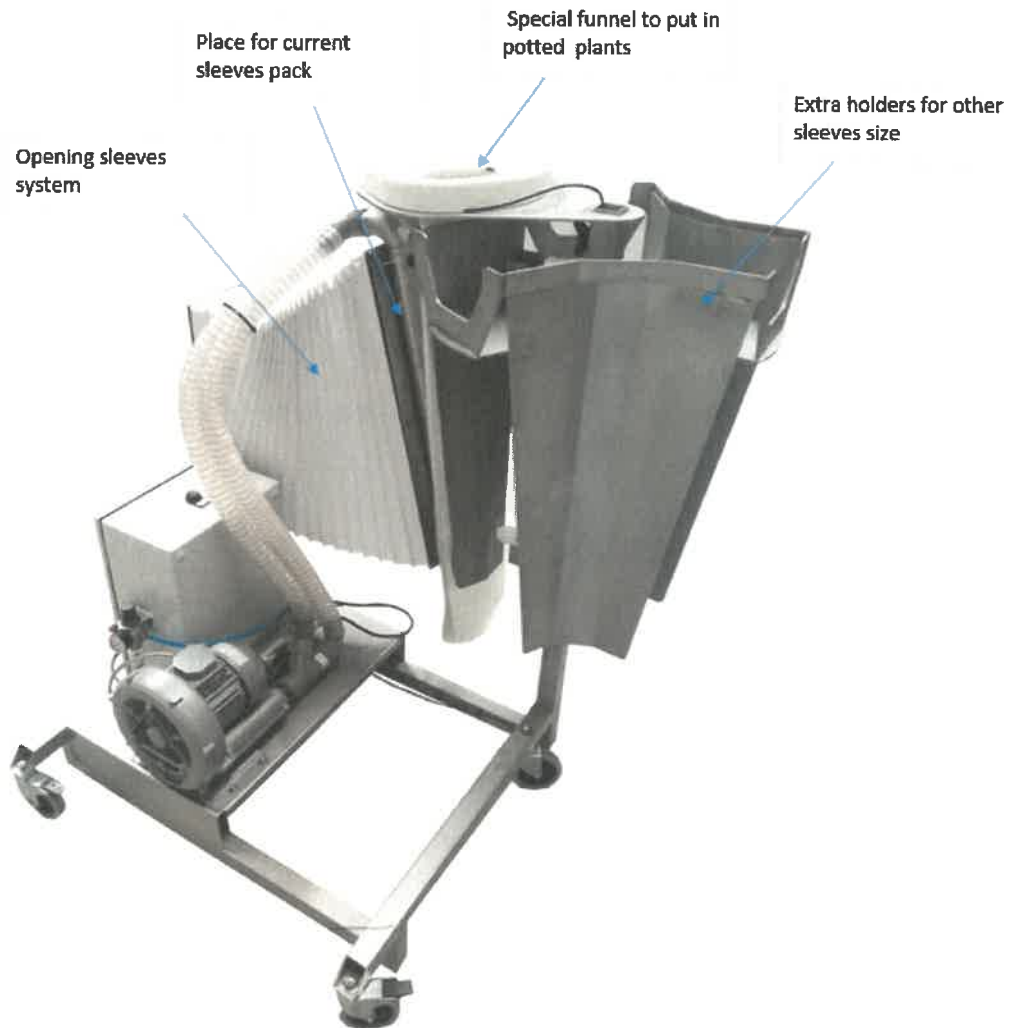
Example and description of the device for packaging potted plants
